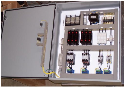
Inside of Typical Large GFI Panel
